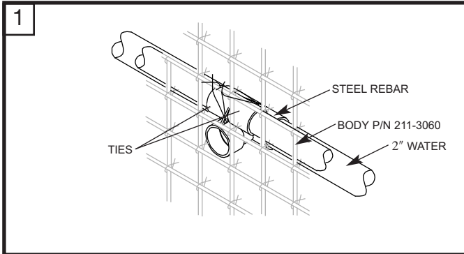
1 Hang Guntie Poly jet Body with ties through preset holes onto steel rebar.
