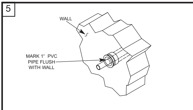
5 Make a mark on the 1" pvc pipe flush or even with the end of the 2 1/2" pipe
