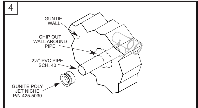
4 After pool guniting scoop around pipe. Before plastering cut the 2-1/2" pvc pipe inside the wall and glue on the Guntie Poly Jet Plaster Niche P/N 425-5030 (not included). Cover niche with tape then plaster over niche.
