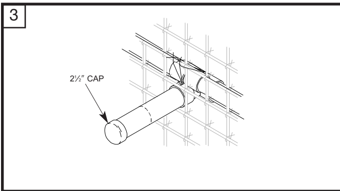
3 Glue 2-1/2" cap onto end of pipe for pressure test before guniting.
