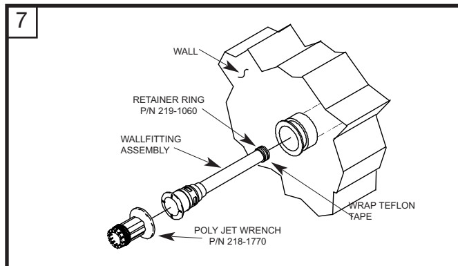
7 Wrap Teflon tape on retainer ring if necessary and thread the 1" PVC pipe back into body with poly jet wrench, making sure of a snug fit.
