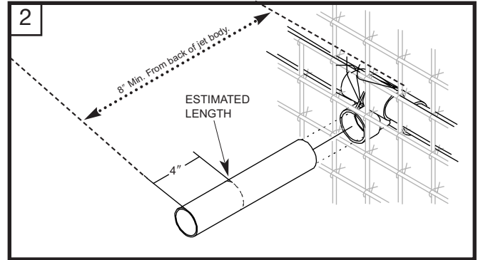
2 Estimate needed length of 2 1/2" pvc pipe by thickness of wall. Cut 2 1/2" pvc pipe at least 4" longer than estimated. Then glue 2 1/2" pvc pie to Body.
