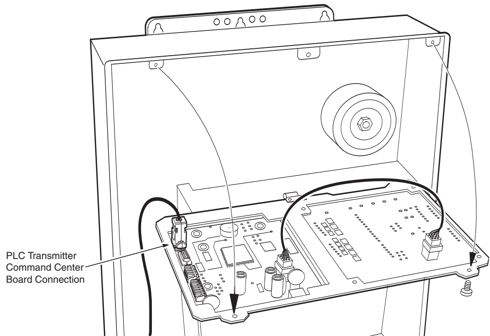
Eos Command Center with hinged board plate down
