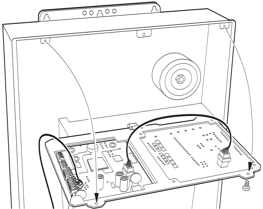
Antenna Connection on Command Center Board
