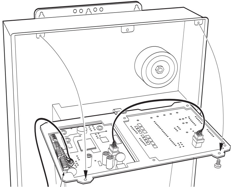
Hub Card Connection on Command Center Board
