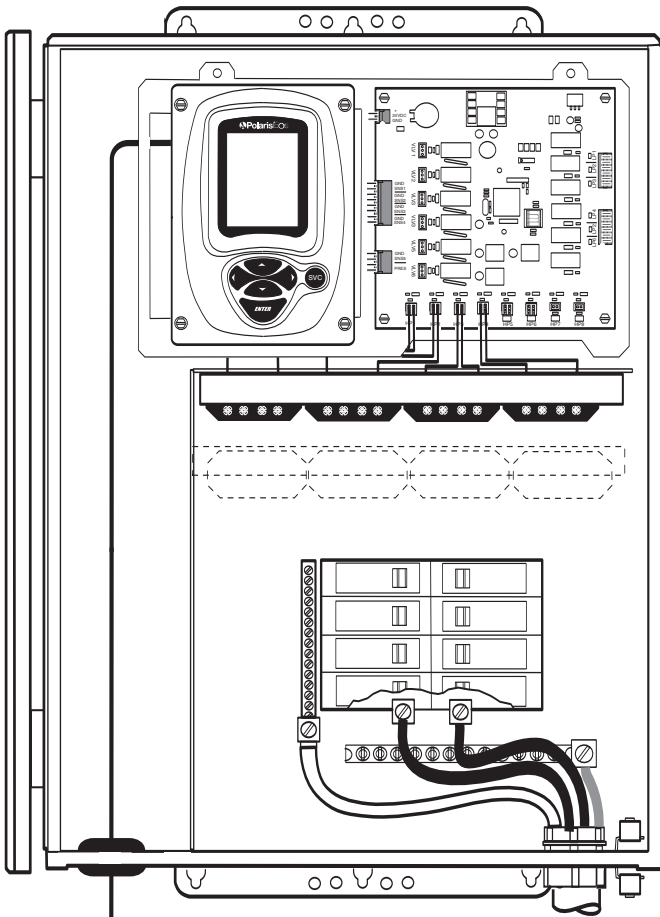
Eos Command Center with hinged board plate down
