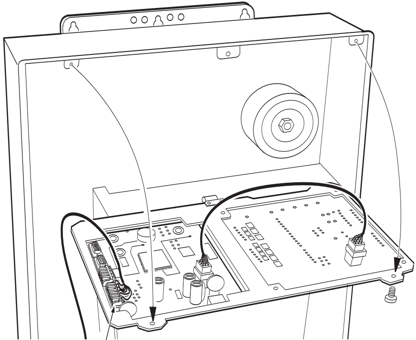
Remote Connection on Command Center Board
