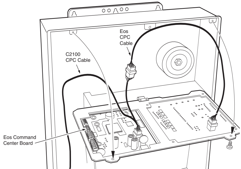
Eos Command Center with hinged board plate down
