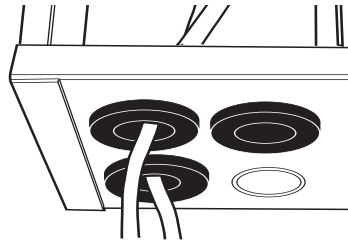
Wiring run through grommets at low voltage compartment
