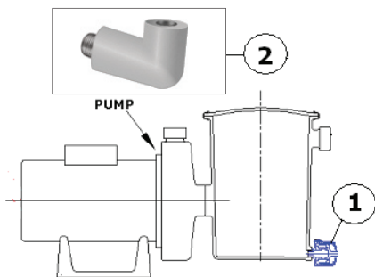
Figure 1. Breather I System Schematic
