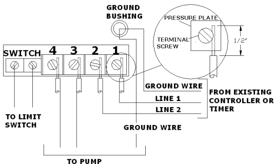
Figure 2. SVRS Box Terminal Layout
