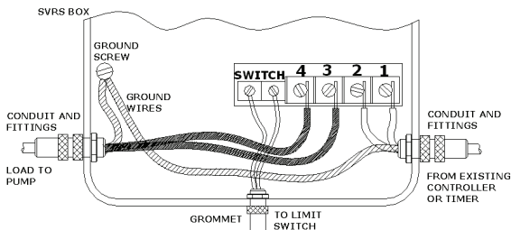
Figure 3. Wiring Diagram
